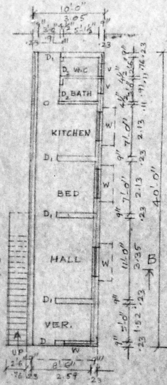
PLAN SCALE:- 1" = 8'-0"
